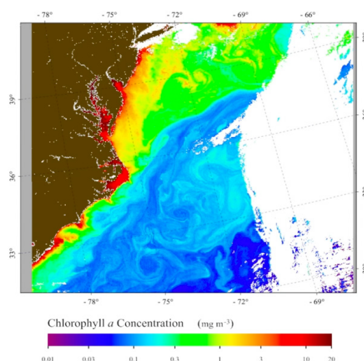
Chlorophyll concentrations in April 2023 for the Chesapeake Bay were created in SeaDAS using Sentinel-3A OLCI Level-2 Earth-observation Full Resolution (EFR) Ocean Color (OC) data.
