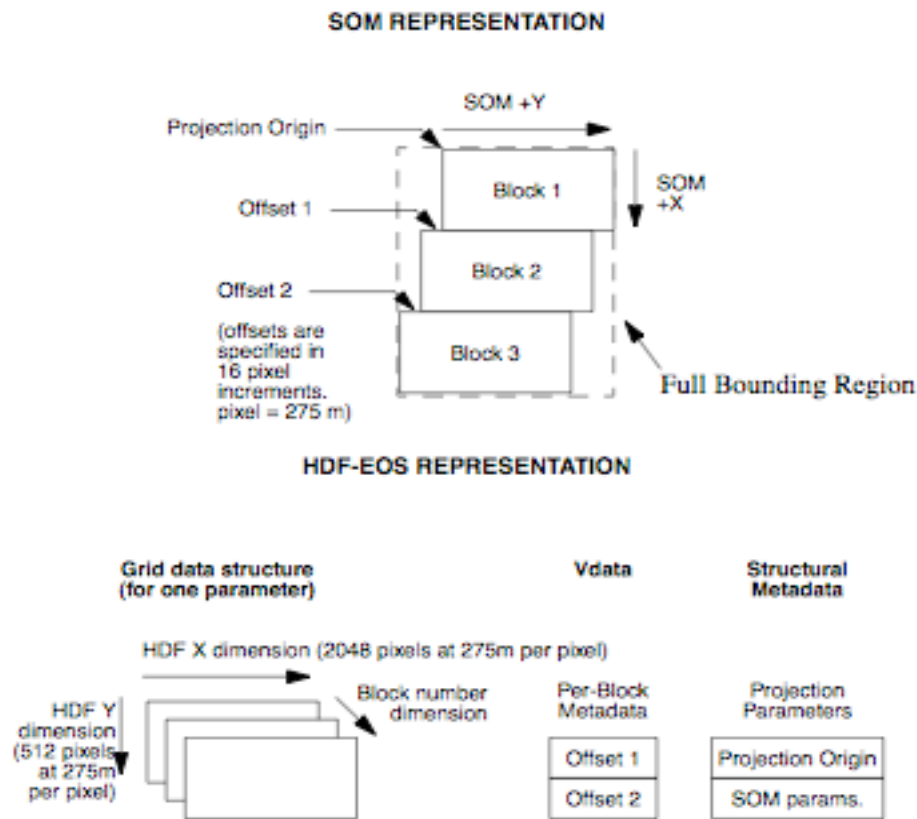
Figure 3-1 MISR SOM Representation in HDF-EOS
