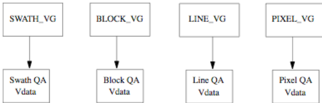
Figure 3-2 MISR QA standard Vdata and Vgroup structures
