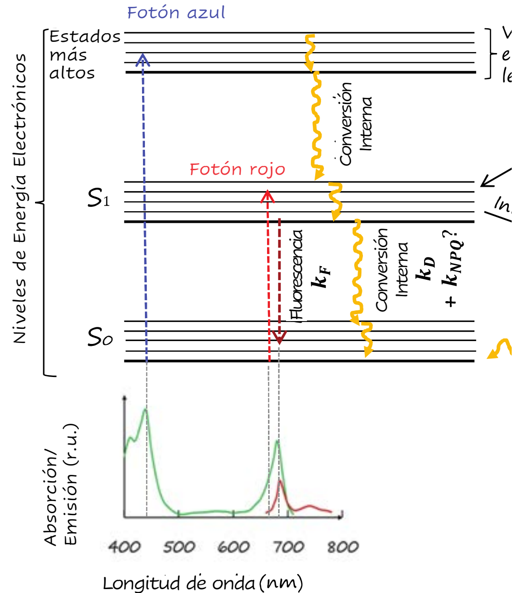
Fig. 3. Idealized Jablonski diagram illustrating the energy partitioning of absorbed blue light, an electron from the ground state is raised to a higher energy state. The Porcar-Castell et al 2014, review initiated at KISS
