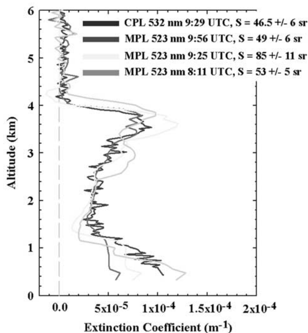
Figure 9. Comparison of extinction profiles from CPL (black profile) and MPL (3 gray profiles) on 29 August 2000 at Skukuza. CPL profile is a 30-s average. MPL profiles are 30-min averages centered at the times listed. Differences in the lowest km are due to aerosol inhomogeneity during the measurements. Altitude is above sea level.
