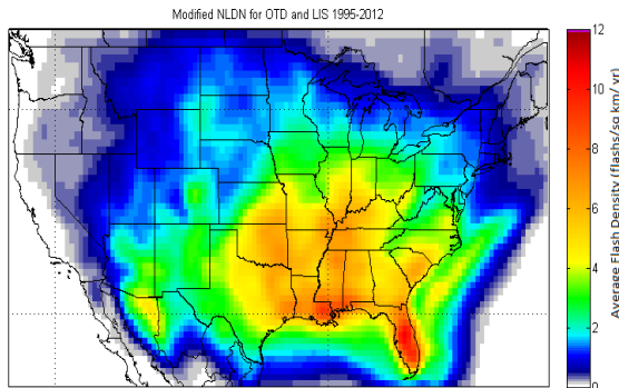
Figure 9: The National Lightning Detection Network’s Ground Flash Density over CONUS where below 38° N the climatology is 17.5 years and above 38° N the climatology is 5 years following OTD.
