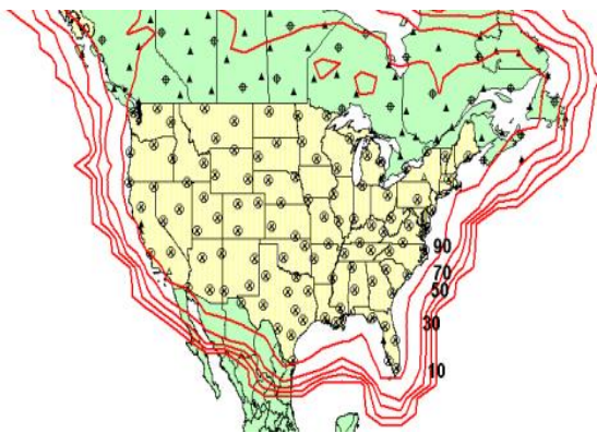
Figure 1: A contour map of the estimated flash Detection Efficiency for the combined NLDN and CLDN since late 1998. Reprinted with permission.
