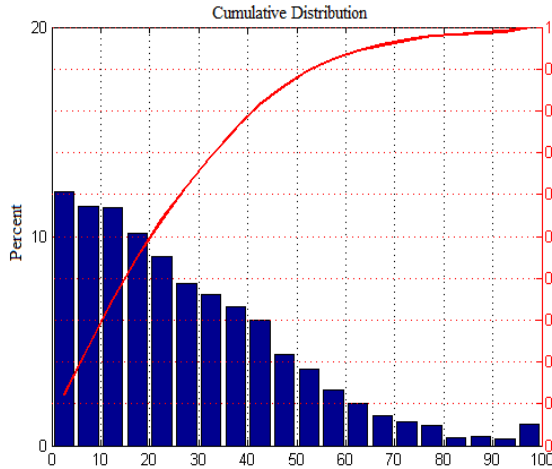
Figure 7: Cumulative sum (line plot) and the histogram (bars) for the magnitude error over CONUS between OTD and LIS.
