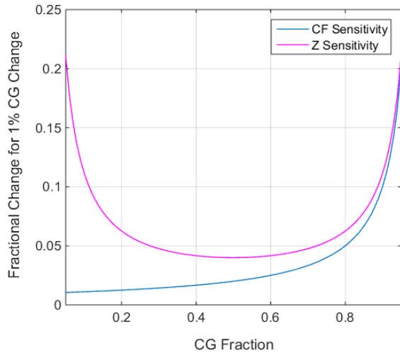
Figure 2: The fractional sensitivity of Z and CF to a 1% change in CG fraction, determined from the derivative of these functions with respect to CG Fraction.
