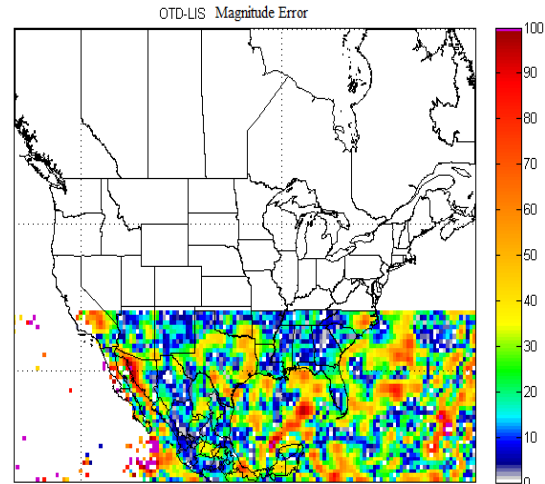
Figure 6: The absolute difference between OTD and LIS flash densities.
