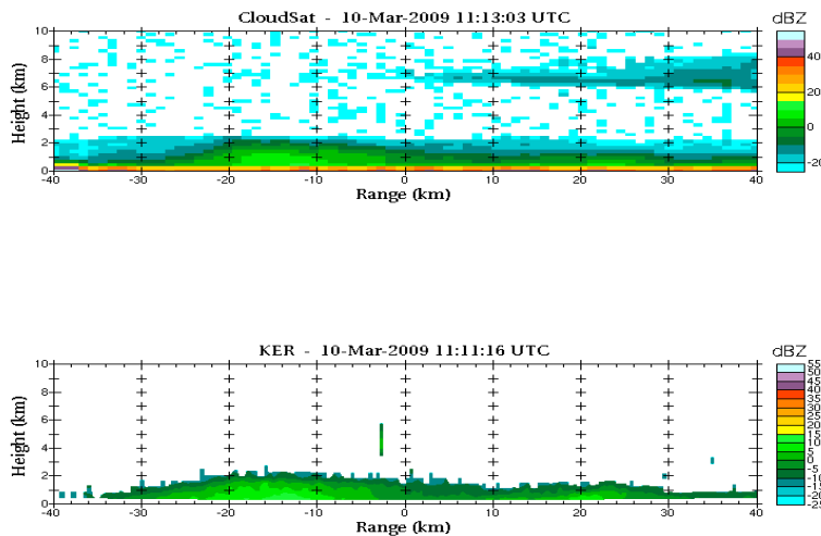
Fig. 5 CloudSat W-band and Kerava C-band radar observations of a snowfall scene in the Gulf of Finland on March 10, 2009. The Kerava observations in the lower panel were extracted along the CloudSat ground track from 3D volume scans since CloudSat does not directly fly over the Kerava radar site.
