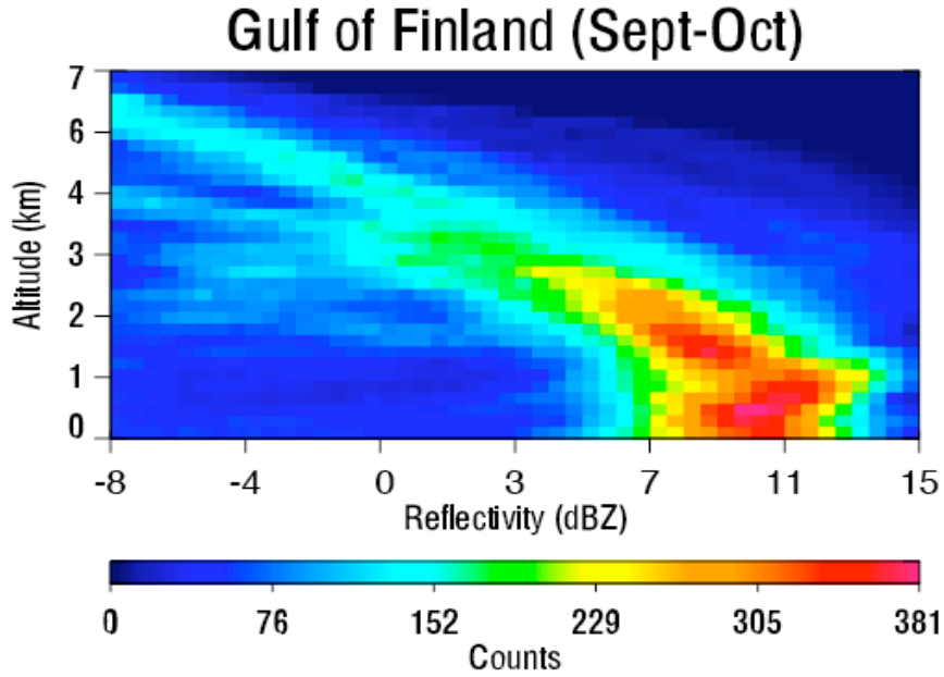
Fig. 2 Reflectivity-altitude histogram of CloudSat CPR observations in the Gulf of Finland during September and October 2007. Reflectivities in excess of 0 dBZ are indicative of precipitation. The peak at ~1 km likely corresponds to the transition from ice to liquid water indicative of the melting layer.
