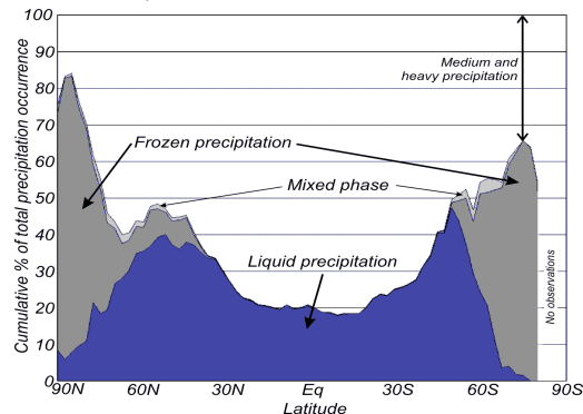
Figure 1 Zonally averaged fraction of precipitation from 1958-1991 falling in the form of light rainfall (less than 1 \text{ mm h}^{-1} ) and snowfall (adapted from the analysis of COADS ship-borne meteorological observations summarized in the EGPM Report for Mission Selection, ESA SP-1279(5)).
